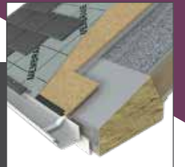
Box beam
